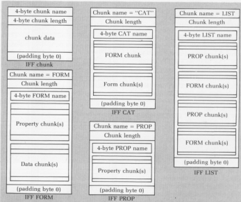
Figure 1: Chunks – the basic building blocks in IFF datafiles
