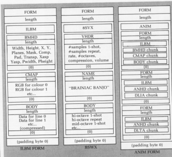
Figure 11: Some examples of FORM chunks
